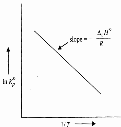
Fig. 7.9.1b Plot of \ln K_p^\circ versus 1/T where \Delta_r H^\circ is positive. Example includes the dissociation of HI into H_2 and I_2
