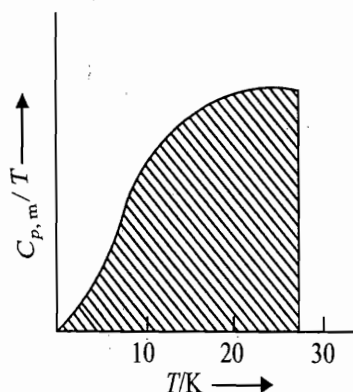
Fig. 4.23.1 Schematic plot of C_{p,m}/T versus T
