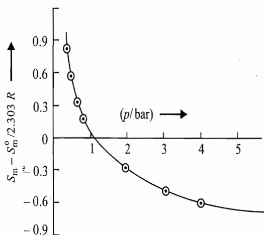
Fig 4.18.1 Plot of S_m - S_m^\circ versus (p/\text{bar})
