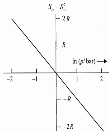
Fig. 4.18.2 S_m - S_m^\circ versus \ln (p/\text{bar})
