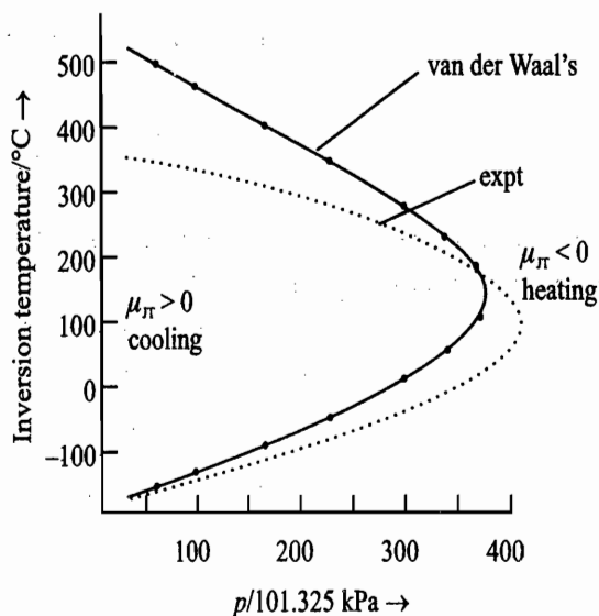
Fig. 2.9.2 A Typical Joule-Thomson inversion curve
