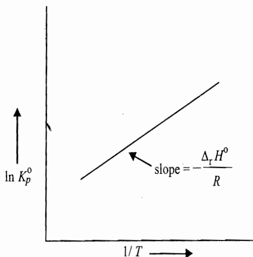
Fig. 7.9.1a Plot of \ln K_p^\circ versus 1/T where \Delta_r H^\circ is negative. Example includes formation of ammonia from N_2 and H_2
