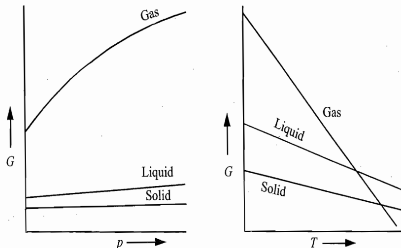
Fig. 5.4.2 Variation of G with T
