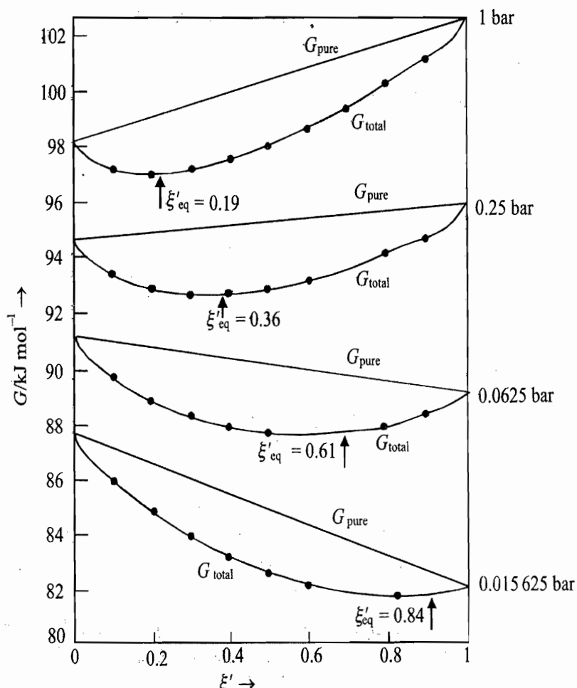
Fig. 7.12.2 Plots of G_{pure} and G_{total} at different pressures
