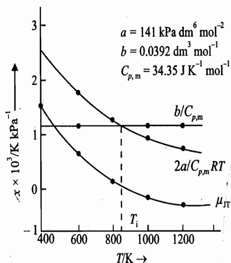
Fig. 2.9.1 The variation of \mu_{JT} and its two components of N_2 (a van der Waals gas) with temperature:
