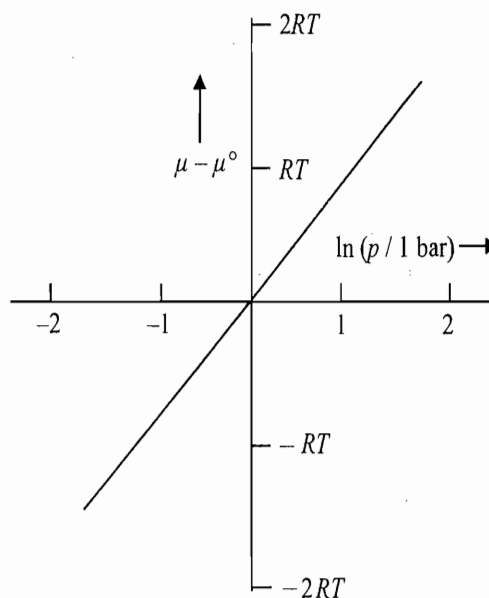
Fig. 5.6.2 Variation of \mu - \mu^\circ for an ideal gas with \ln (p/1 \text{ bar})
